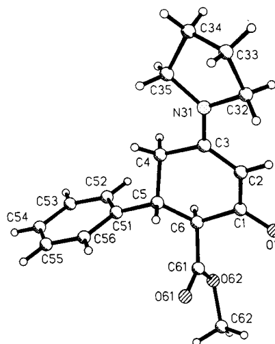
Figure 2. Perspective view and atom labelling of 2m .
